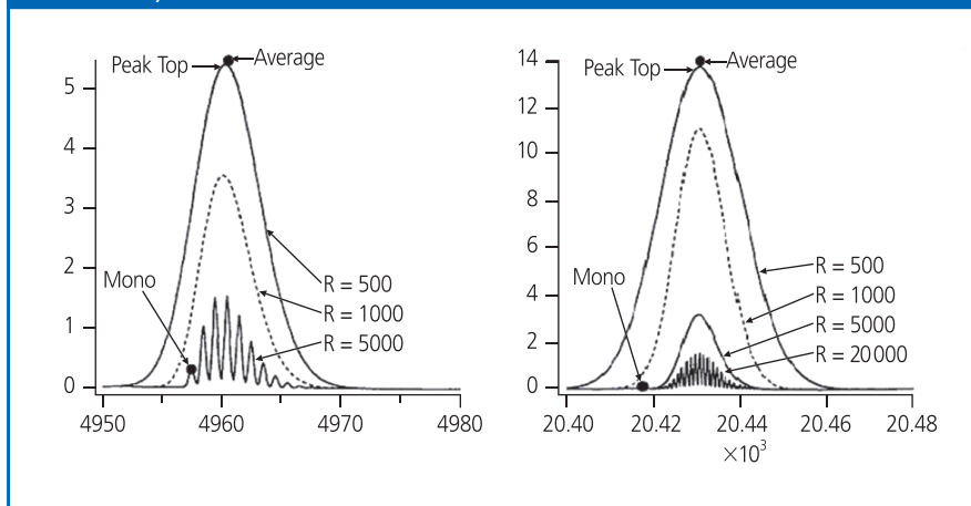
Figure 4: Although spectral features are discerned only as mass increases when the resolution is sufficient, the "composite" envelope (and hence the difference between the peak top and the average mass value) is less pronounced. (Adapted from reference 8.)
