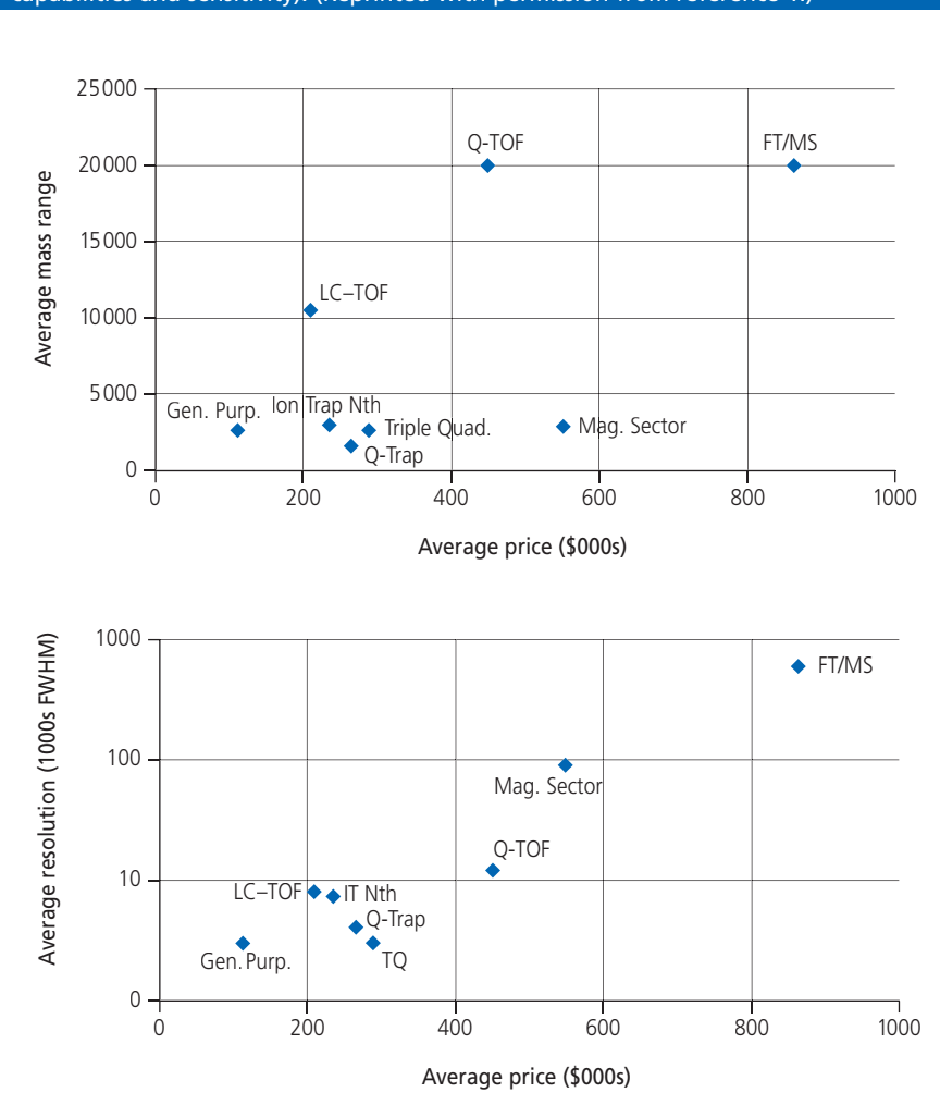
Figure 5: Differentiated by overall cost (and complexity), the combination of quadrupole technology and TOF appears to deliver the best capability, especially in terms of performance (fragmentation for structural characterization, quantitative capabilities and sensitivity). (Reprinted with permission from reference 1.)
