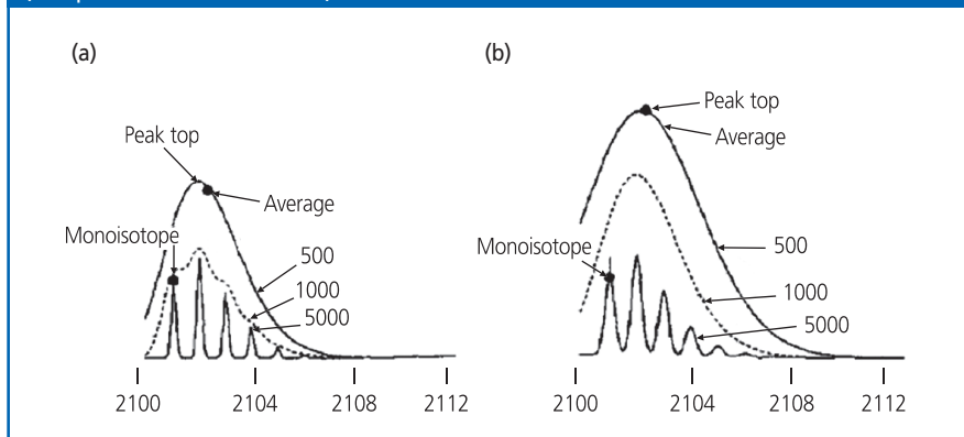
Figure 3: Comparison of resolution values and the consequent ability to discern spectral features using (a) the 10% valley method and (b) the FWHM method. Analyte: bradykinin dimer [ C_{100}H_{144}N_{30}O_{21} with a nominal mass of 2100]. (Adapted from reference 8.)
