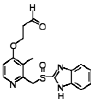
Aldehyde
